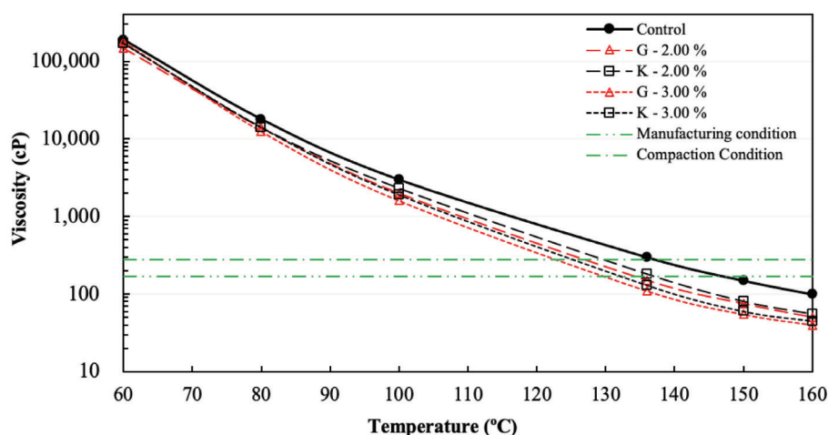
Figure 2. Viscosity results of asphalt binder
