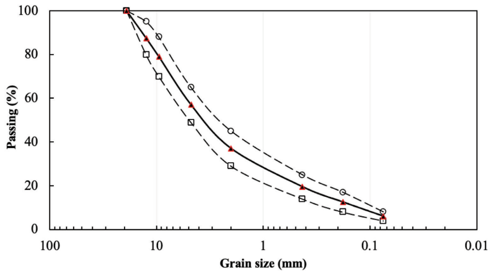
Figure 1. Gradation curve used in the preparation of specimens
