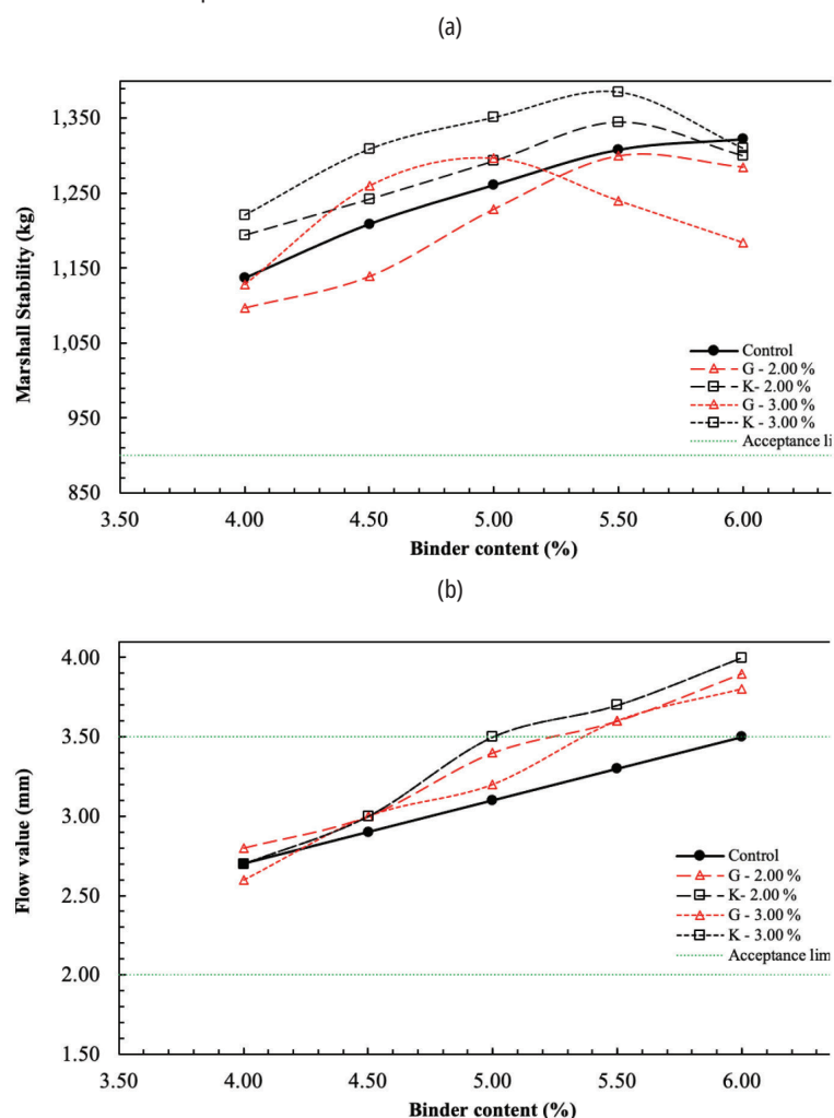
Figure 4. Evaluation of mechanical parameters
