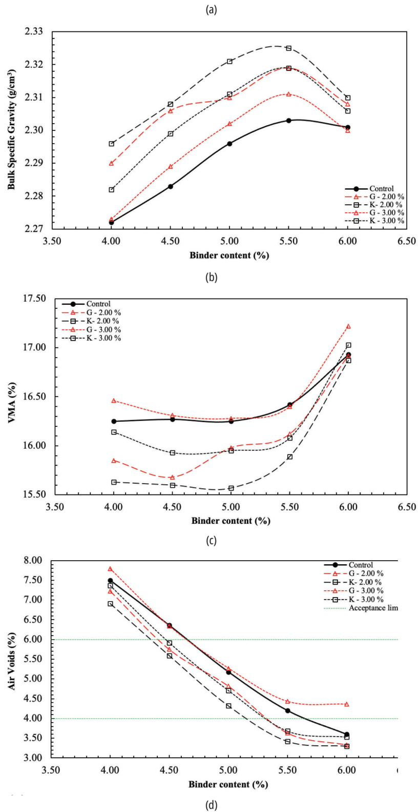
Figure 3. Bulk Specific Gravity and volumetric properties of the mixtures
