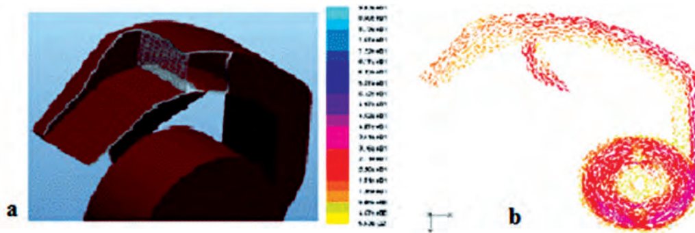
FIGURE 7. Simulation of mill of hammers with device of sifting. a) Design of the device of sifting, b) Distribution of air flow for CFD.
