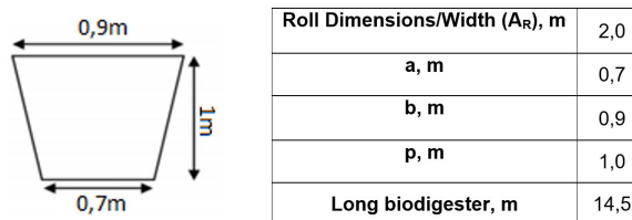
FIGURE 4. Main dimensions of the trench and the proposed polyethylene tubular biodigester.
