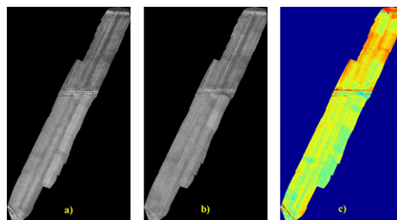
FIGURE 2. Orthomosaics constructed using the MSI of the a) NIR and b) RE bands of the MicaSense camera. c) Result of image processing, highlighting in orange the highest infection and in green the no brown rust infection.
