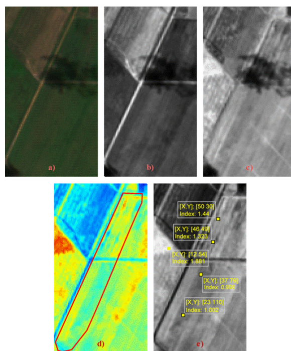
FIGURE 3. Images obtained by Sentinel-2. a) True color (RGB), b) and c) bands 4 and 8, d) calculated index in pseudo color and e) calculated index showing some values.
