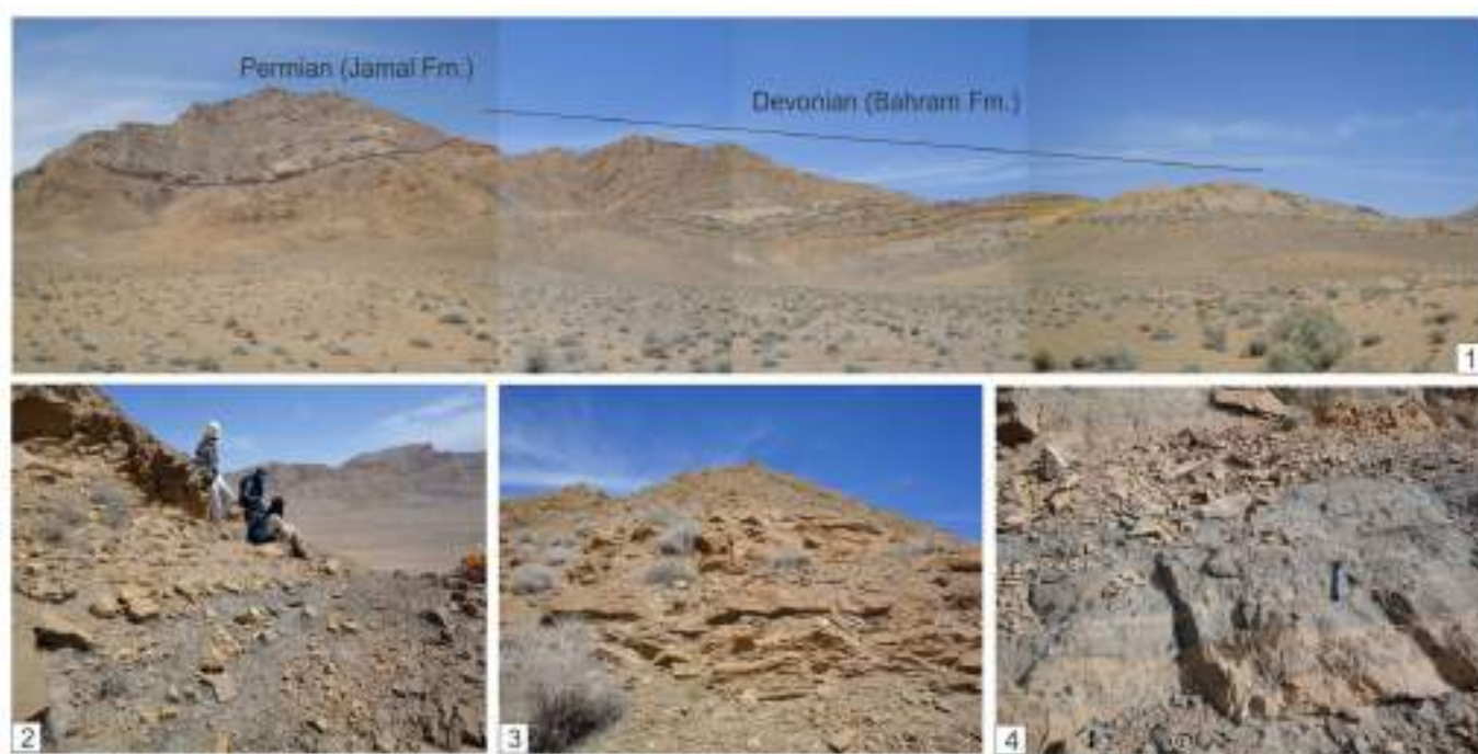
Figure 2 Representative examples of different shallow-water sediments from the investigated sections. (1) Panoramic view of the Baqer-Abad section. (2) Grey to black shale (package 8, Figure 4) at the upper part of the studied profile. (3) Sandy dolomitic limestone (see package 7, Figure 4). (4) Alternation of yellow to grey limestone with algal contents (upper part of package 1, see Figure 4).
