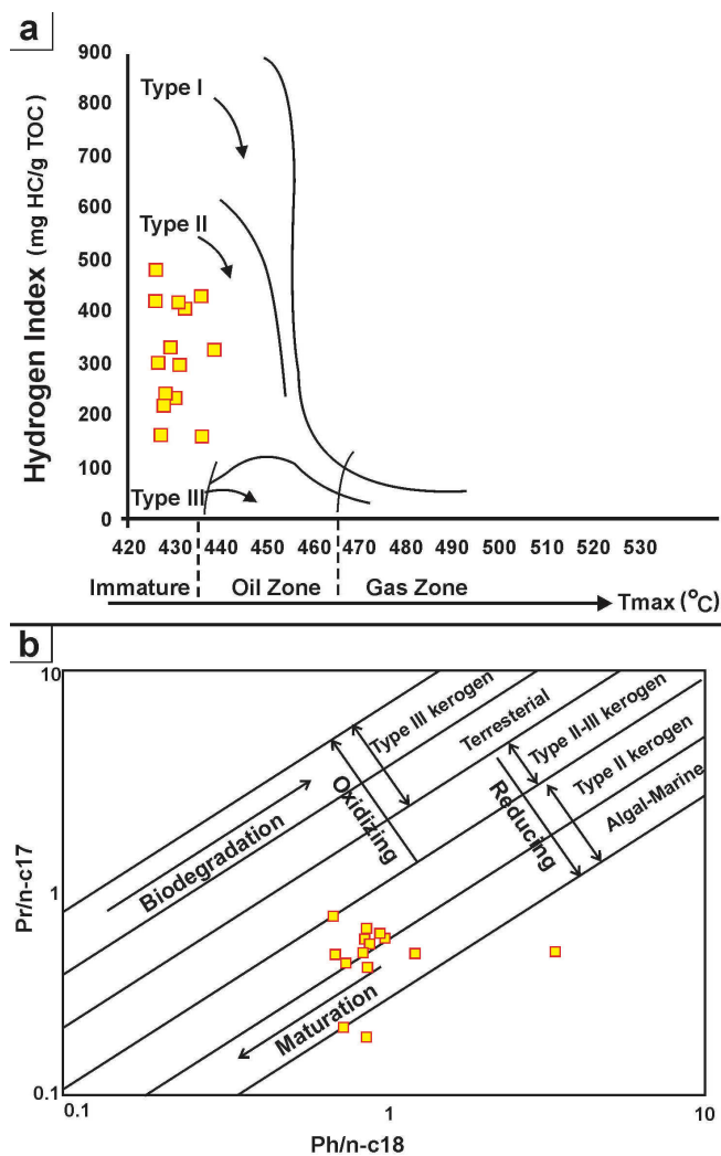
Figure 6 a) HI versus Tmax diagram for the Pabdeh Formation samples. b) Cross-plot of Pr/n-C 17 versus Ph/n-C 18 for the Pabdeh Formation samples.
