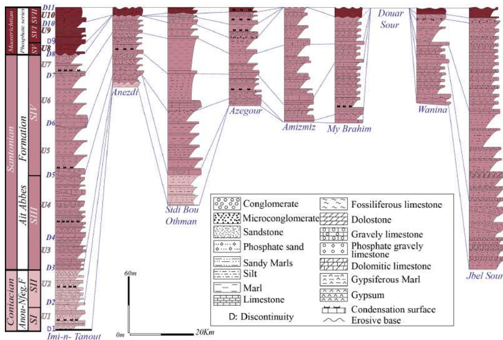
Figure 6 Lithostratigraphic correlations.
