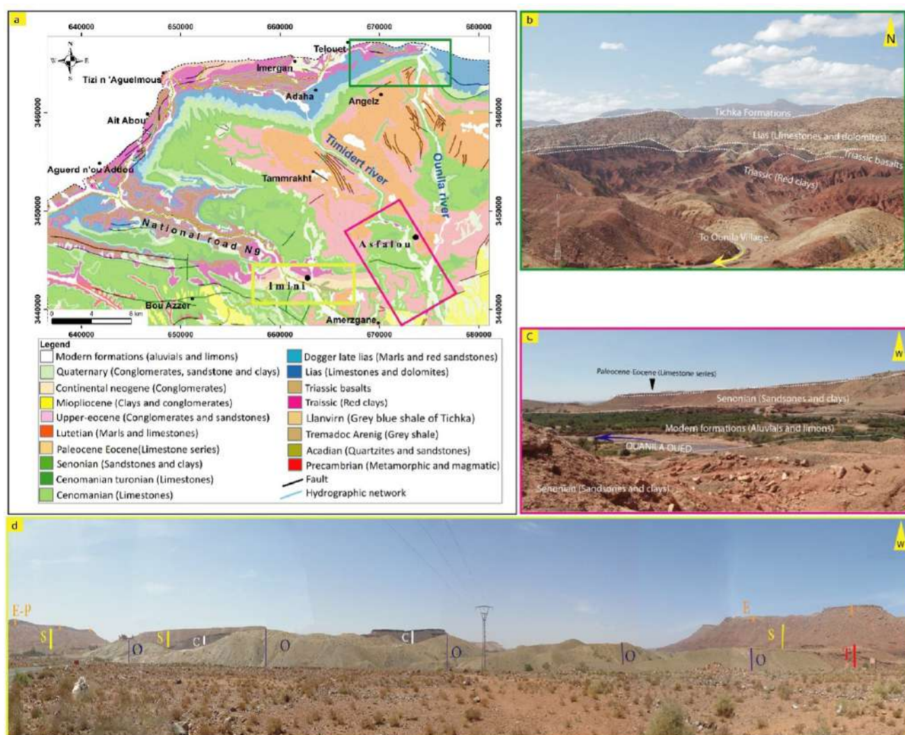
Figure 2 (A) Litho structural map extracted from the geological map of Ouarzazate Alougoum at 1/100000. (B) Panoramic view in the Anmitar district. (C) Panoramic view in the Asfalou district. (D). Panoramic view in the Imini district. (E-P: Eocene Paleocene, S: Senonian, O: Ordovician, C: Cretaceous, E: Eocene, T: Triassic).
