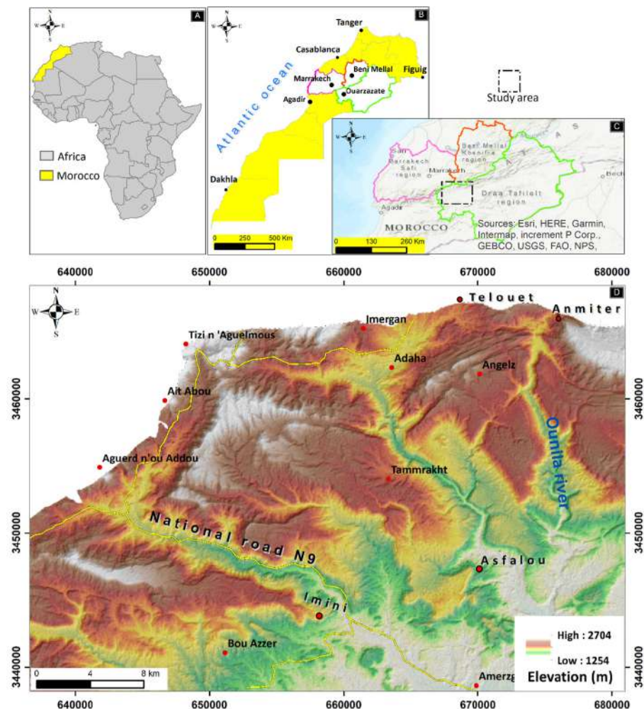
Figure 1 Location of the study area: (A) African view, (B) National view, (C) Regional view, and (D) 2D elevation map of the study area.
