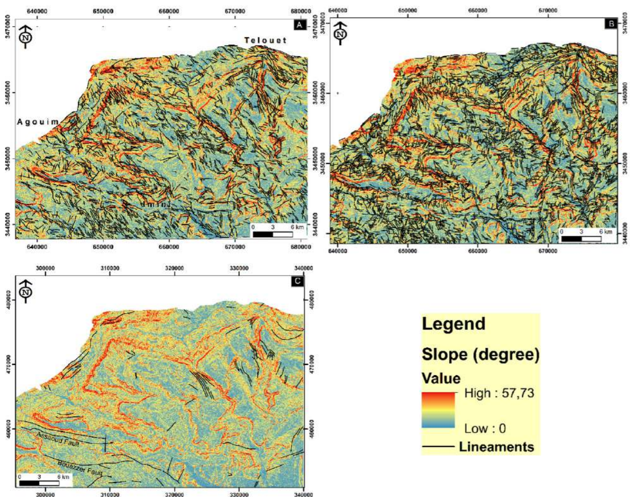
Figure 12 Overlay of the slope image and resulting lineament maps from the PC1 image (A), the DEM image (B), and the Geological map (C).
