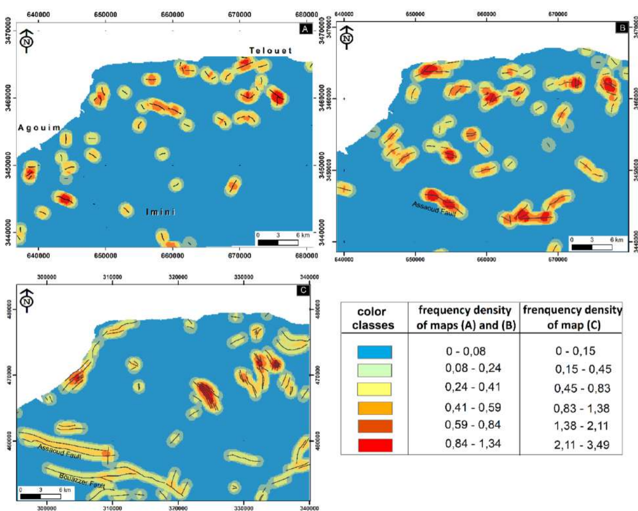
Figure 11 Lineament density map of lineaments extracted from (A) PC1 image, (B) DEM image, and (C) Geological map.
