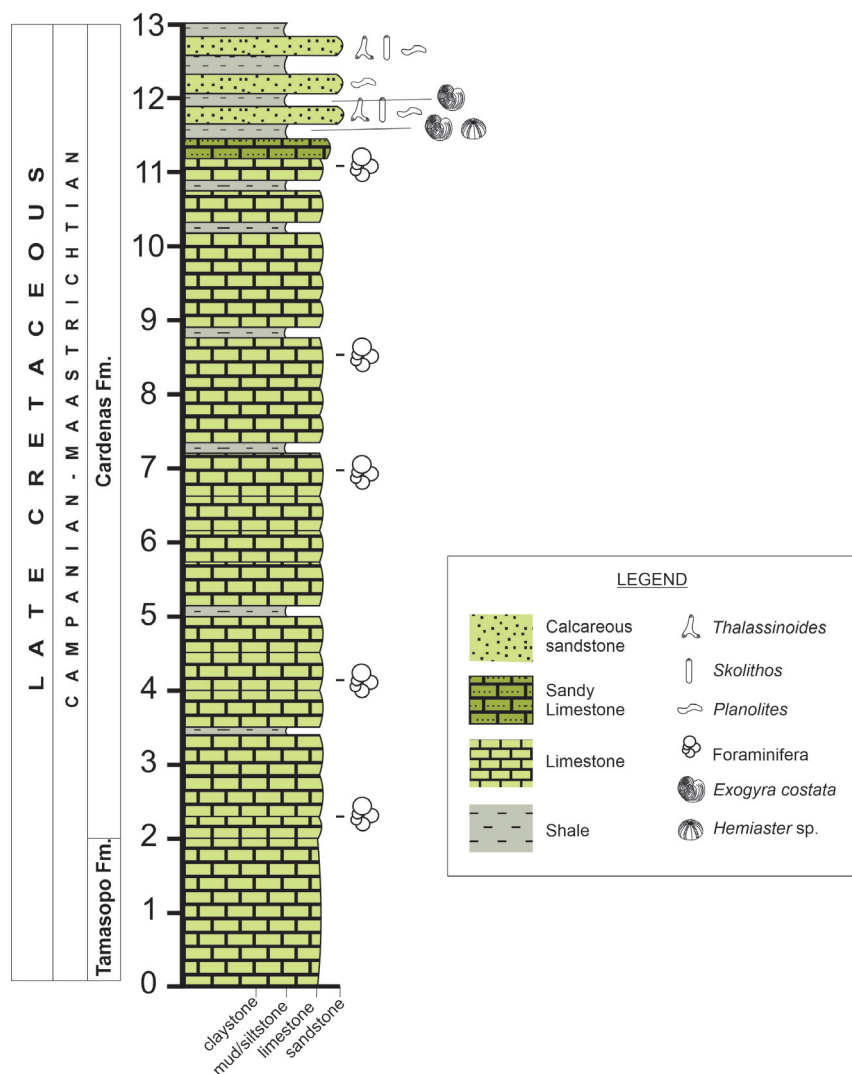
Figure 2 Stratigraphic section of the Cárdenas Formation in Potrero del Carnero outcrop. Notice that trace fossils just crop near to the top of the studied section.
