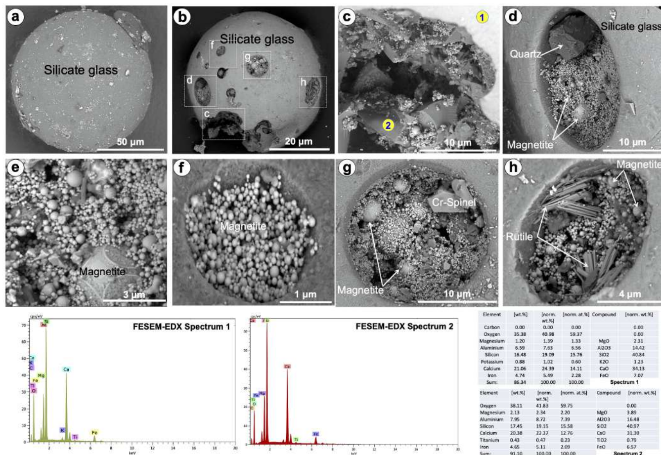
Figure 4 Microphotographs collected by FESEM in SE mode of the glassy spherules recovered from the Yakovitsa (a) and Golyamo Kameneniyane (b-h) chromitites. Representative FESEM-EDX spectrum of the glass are inset in the figure.
