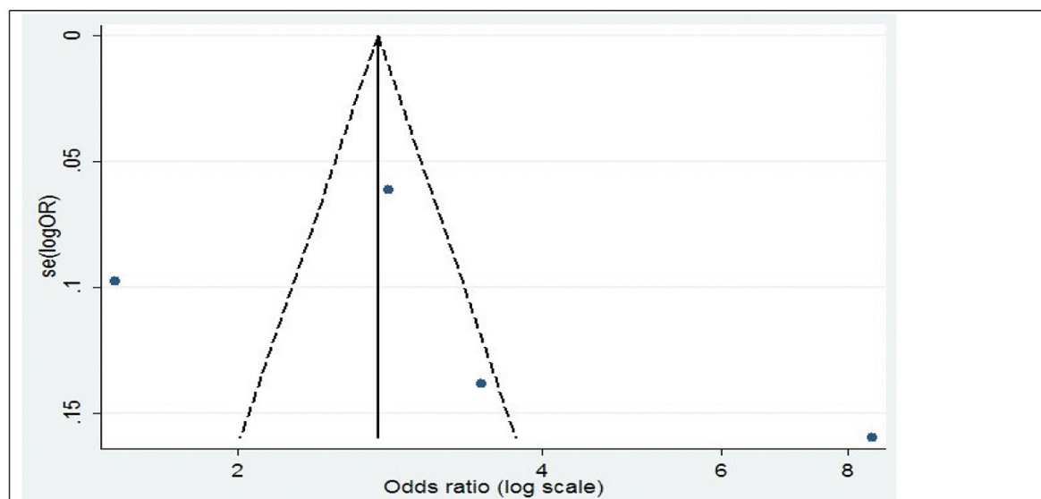
Figura 4. Funnel plot.
