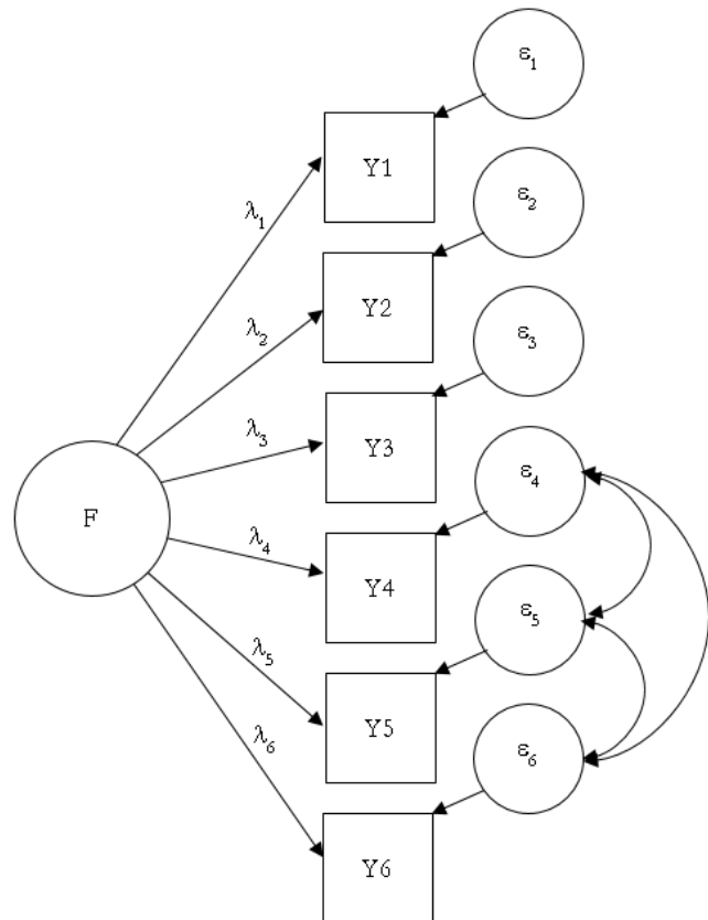
Figure 2. Model of essentially tau-equivalent measures on the left, measurement model with correlated errors between three items on the right.
