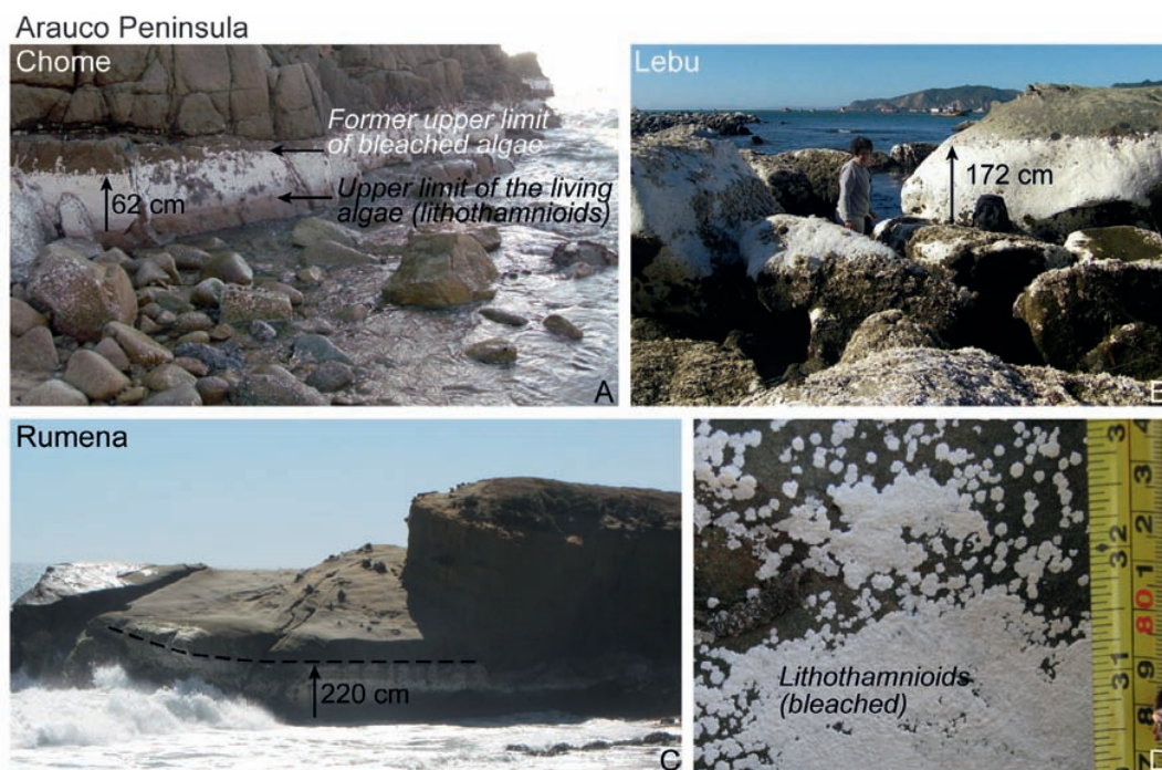
FIG. 2. Bleached lithothamnioids coralline algae strip used as a marker of coastal coseismic uplifting. A. , B. Pink (living) algae strip and white fringe of the crustose coralline algae observed at Chome and Lebu, respectively; C. White fringe of bleached algae at Rumena, showing increased width in the zone directly exposed to the waves; D. Detail of bleached lithothamnioids algae as a result of coastal coseismic uplift during the 2010 Maule earthquake.
