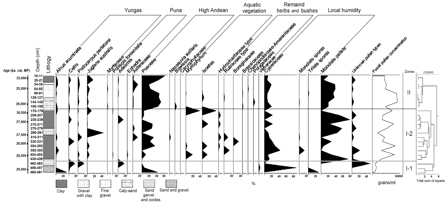
FIG. 4. Fossil pollen diagram of TLB-1 core.
