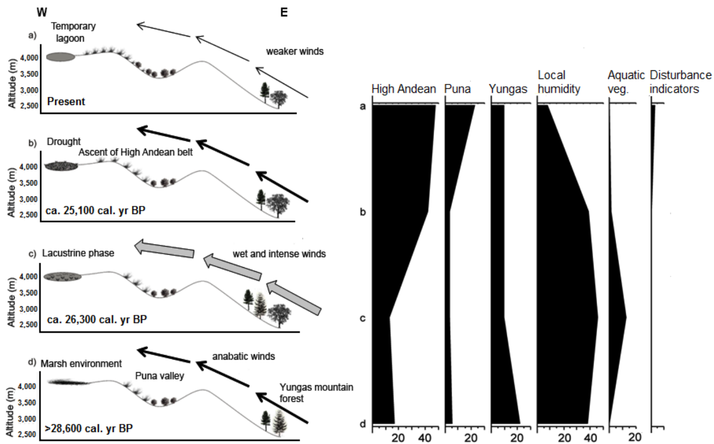
FIG. 5. Inferred vegetation change during the Pre-LGM at Laguna Blanca.
