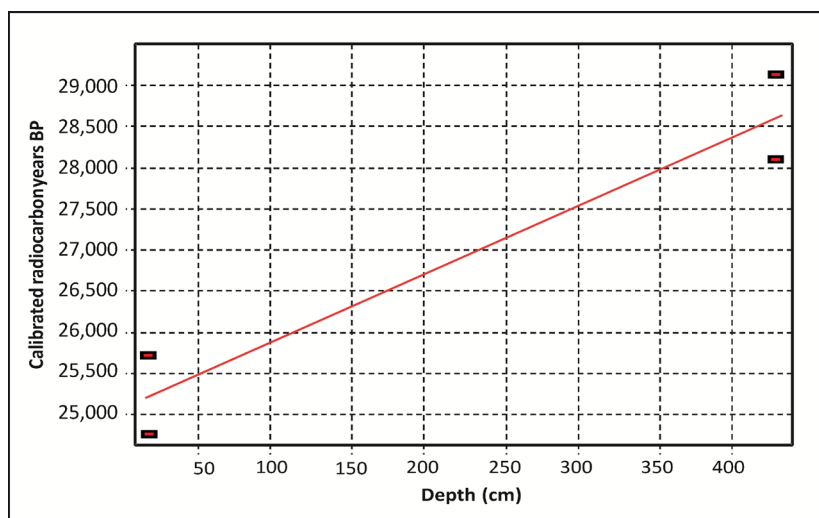
FIG. 3. Age-depth model for Laguna Blanca sediment core.
