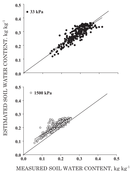
Figure 5. Ratio between the gravimetric soil water content measured for the soils of the irrigation system ( \theta_{gml} ) and that estimated by the proposed model ( \theta_{ges} ) for soils with particle size distribution information.
