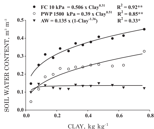
Figure 7. Relationship between the clay content in the soil and the water content at field capacity (FC = 10 kPa), at the permanent wilting point (PWP = 1,500 kPa) and the plant-available water capacity (AW = different between water content at 10 and at 1,500 kPa) for the RS soils.
