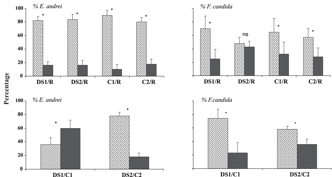
Figure 1. Avoidance response of earthworms ( Eisenia andrei ) and springtails ( Folsomia candida ) in different tested soils. C1 and C2: fields treated with conventional fertilization. DS1, DS2: Fields treated with sludge as of May 2004 (DS1), May 2005 (DS2). R: reference soil. Values are the average percentage of organisms found on control or tested sides. Vertical lines represent standard deviation. *: significantly higher percentage of organisms on the control side than on the tested side ( p < 0.05 ).
