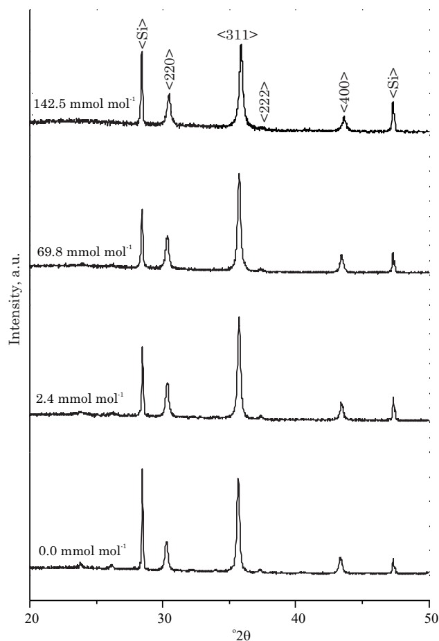
Figure 1. X-ray diffraction patterns for the Al-substituted maghemites. Si: silicon as internal standard.
