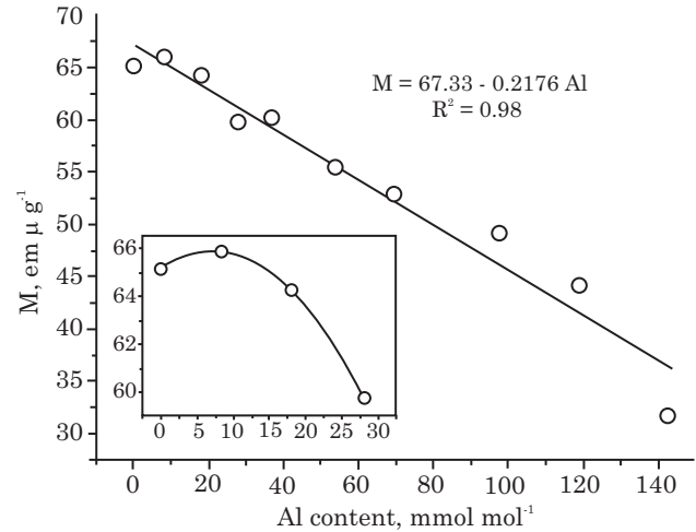
Figure 6. Magnetization at 10 kOe as function of isomorphous substitution of \text{Fe}^{3+} for \text{Al}^{3+} in synthetic substituted maghemite.
