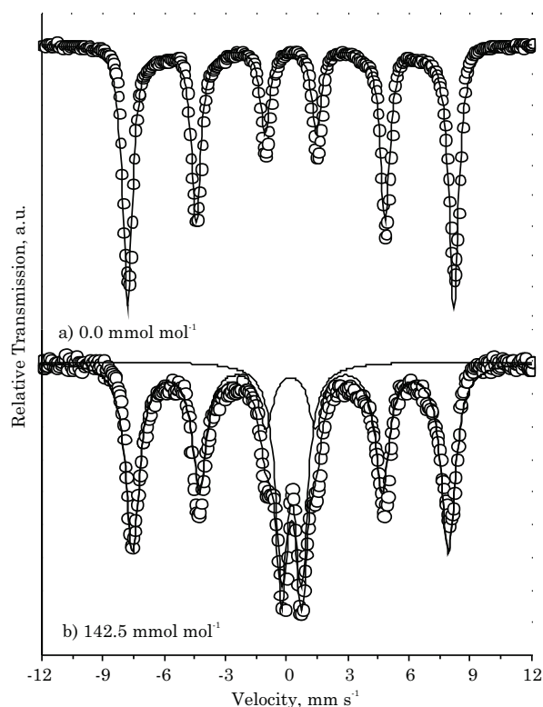
Figure 3. RT Mössbauer spectra for pure maghemite (a) and with 142.5 \text{ mmol mol}^{-1} (b) of isomorphous substitution of \text{Fe}^{3+} for \text{Al}^{3+} .
