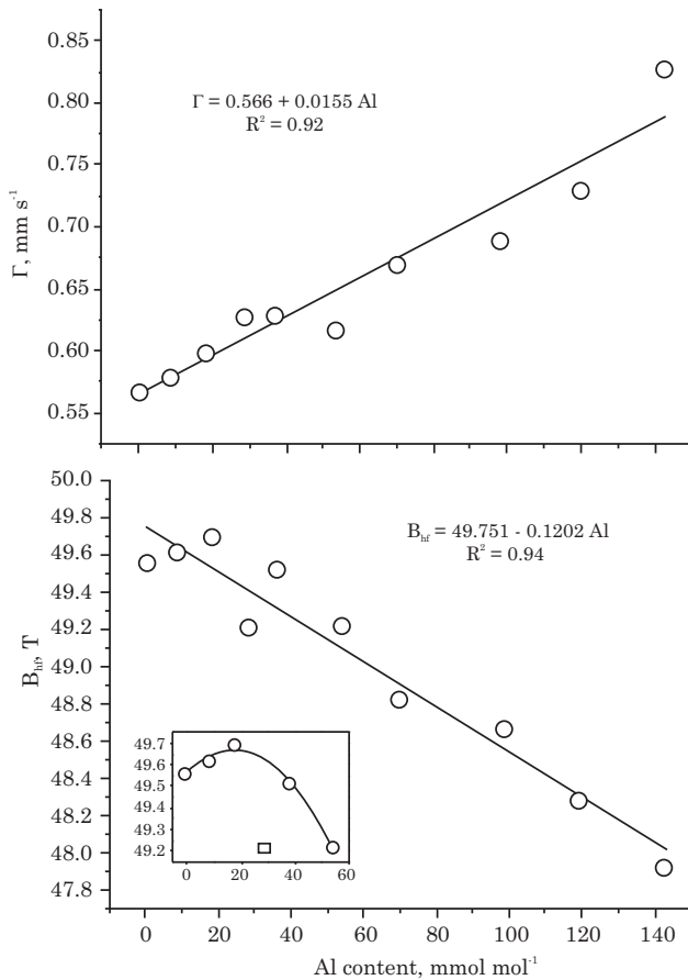
Figure 4. Linewidth ( \Gamma ) of the Mössbauer spectra (a), and hyperfine magnetic interaction ( B_{hf} ) (b) for synthetic aluminum substituted maghemite. (□) Outlier.
