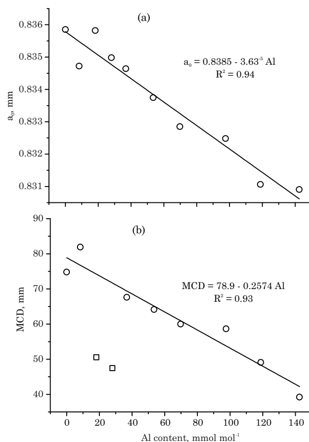
Figure 2. Average lattice parameter ( a_0 ) for the Al-substituted maghemite (a), and mean crystalline diameter for the Al-substituted maghemites (b), as a function of aluminum content. (□) Outlier.
