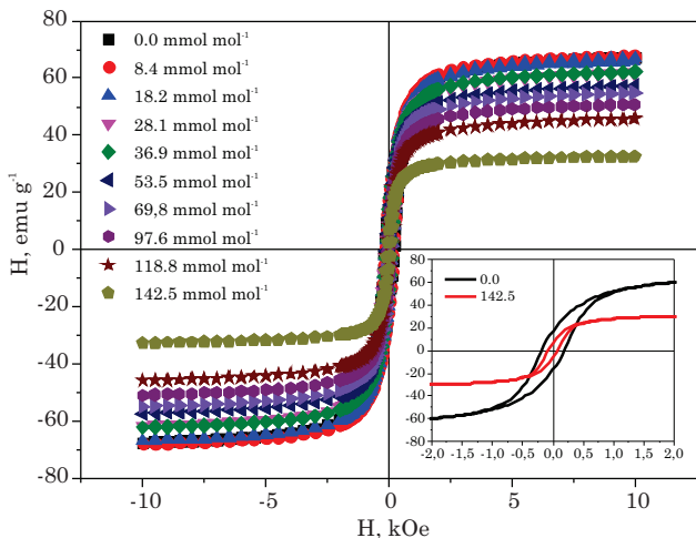
Figure 5. Magnetic hysteresis loops for \gamma\text{-Fe}_{2-x}\text{Al}_x\text{O}_3 samples at RT; Insets: 0.0 and 142.5 \text{mmol mol}^{-1} Al-substituted maghemites.
