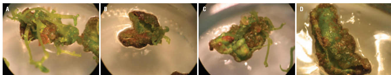
FIGURE 3. Regeneration of transformed Pastusa Suprema leaf explants in regeneration medium RM media supplemented with kanamycin 100 mg L -1 A, Calli produced 3 weeks after transformation. B, Regeneration of shoots at 5 weeks after transformation. C, Stems grown at 6 weeks. D, Regeneration after 8 weeks. Source photographs: Torres, E.S.
