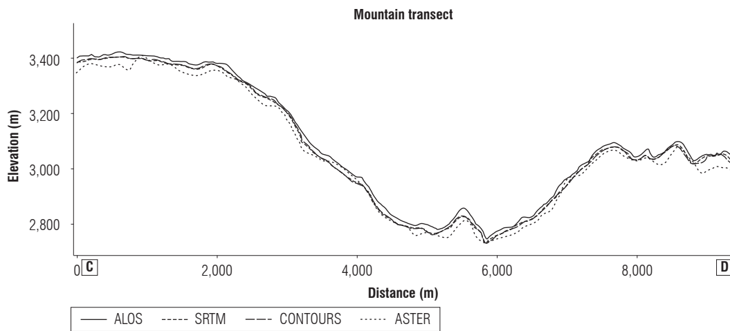
FIGURE 3. Transect to the mountain landscape with different DEMs in a Samaca area (Colombia).
