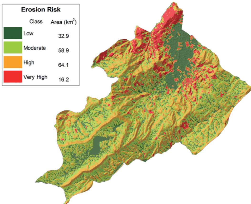
FIGURE 6. Erosion risk for a Samaca area (Colombia).
