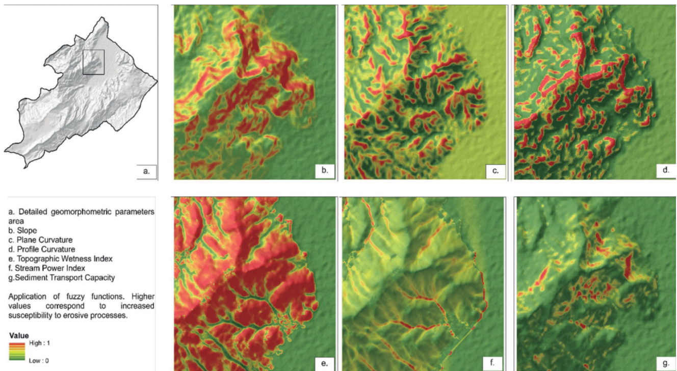
FIGURE 5. Results of fuzzy logic functions in the terrain parameter in a Samaca area (Colombia).
