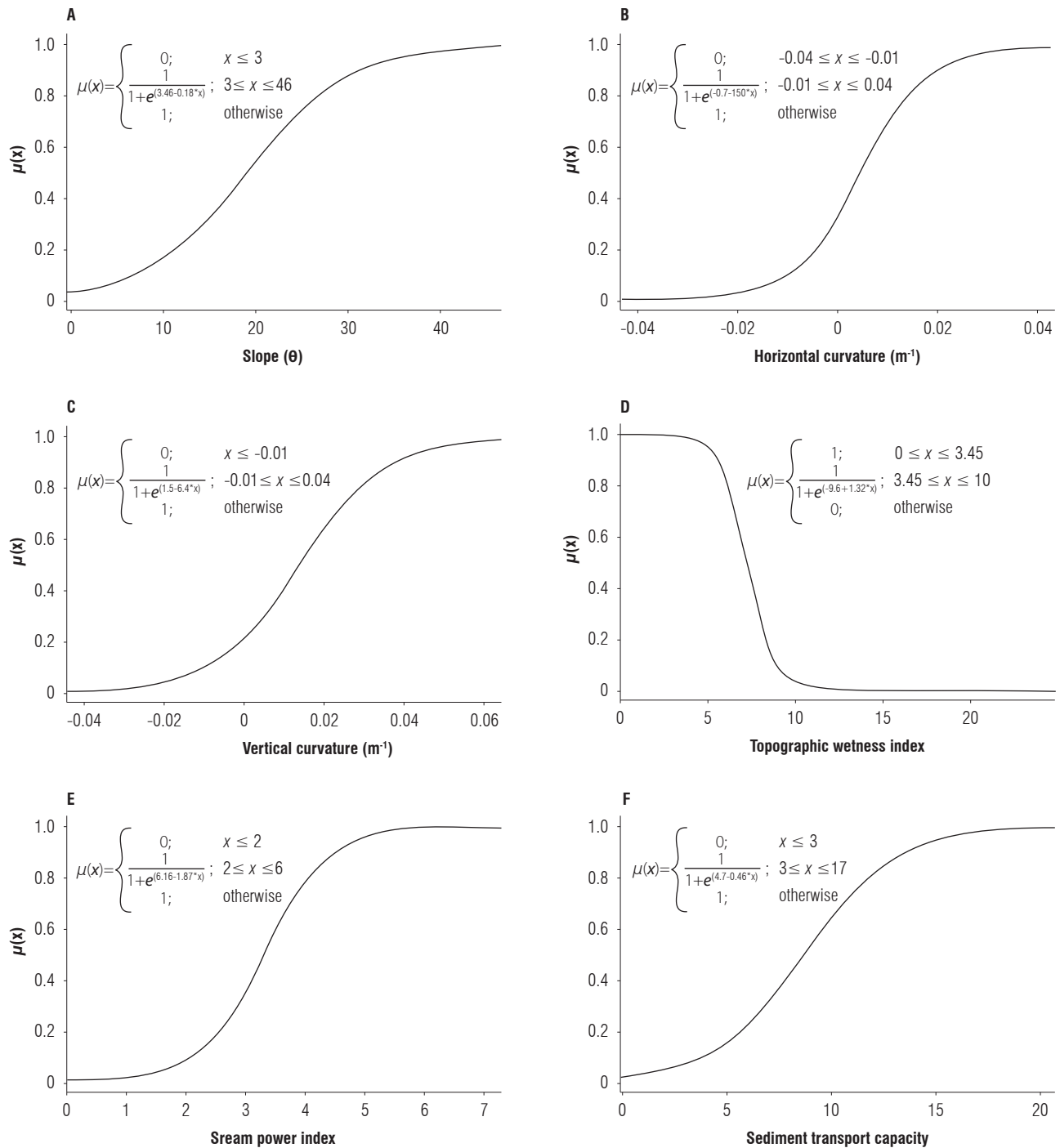
FIGURE 4. Fuzzy logic functions applied to terrain parameters in a Samaca area (Colombia).
