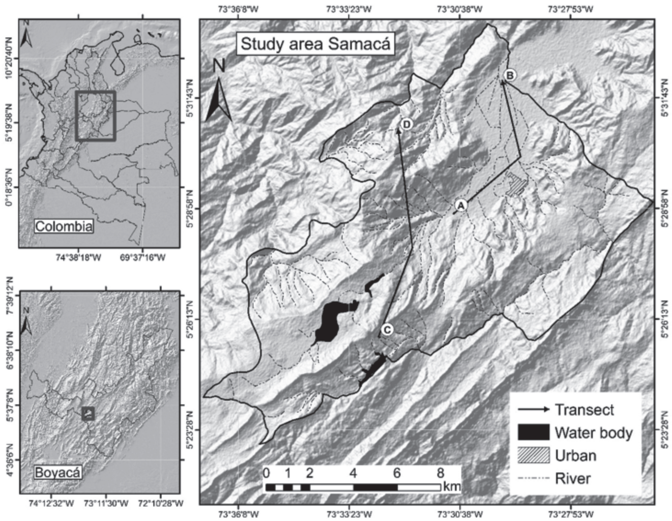
FIGURE 1. Location and transect of landscape for the study area in Samaca (Colombia).
