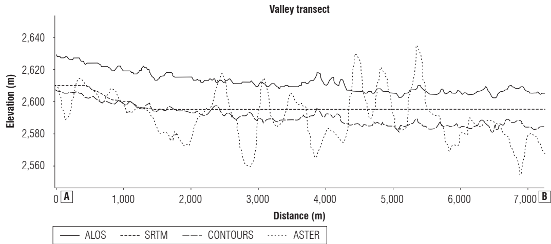
FIGURE 2. Topographic profile to the valley with different DEM's in a Samaca area (Colombia).
