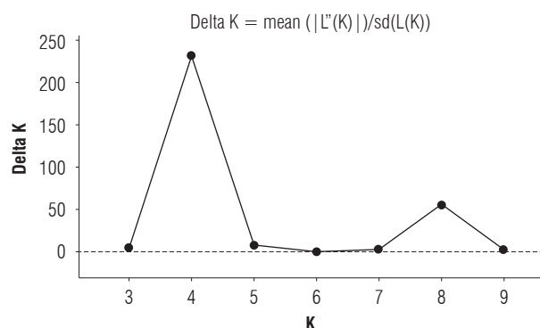
FIGURE 3. Delta K values compared to the number of groups ( K ) in the 102 yellow passion fruit individuals.
