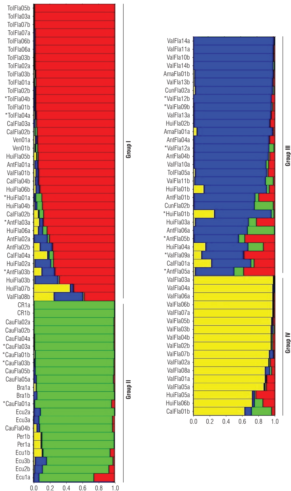
FIGURE 4. Bayesian analysis of the genetic structure ( K=4 ) in the 51 yellow passion fruit accessions based on six microsatellite loci. Each bar represents one individual genotype, and individuals with multiple colors have admixed genotypes from multiple clusters. Elite accessions identified by Ocampo et al. (2013) are indicated with an asterisk (*).
