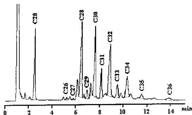
Figure 1: Gas-chromatogram of the mixture of alcohols obtained from Agave furcroydes L. wax
