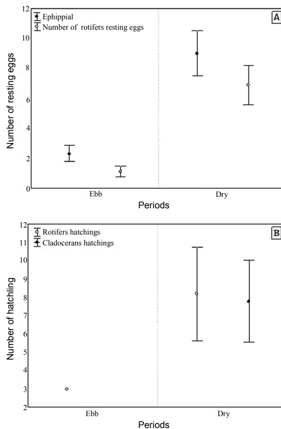
Figure 3. Temporal variation in the number of resting eggs of zooplankton organisms found (A) and in the number of hatchlings from these eggs (B), in the period from May to November 2008. (symbol = mean of the sampling months and bar = standard error).
