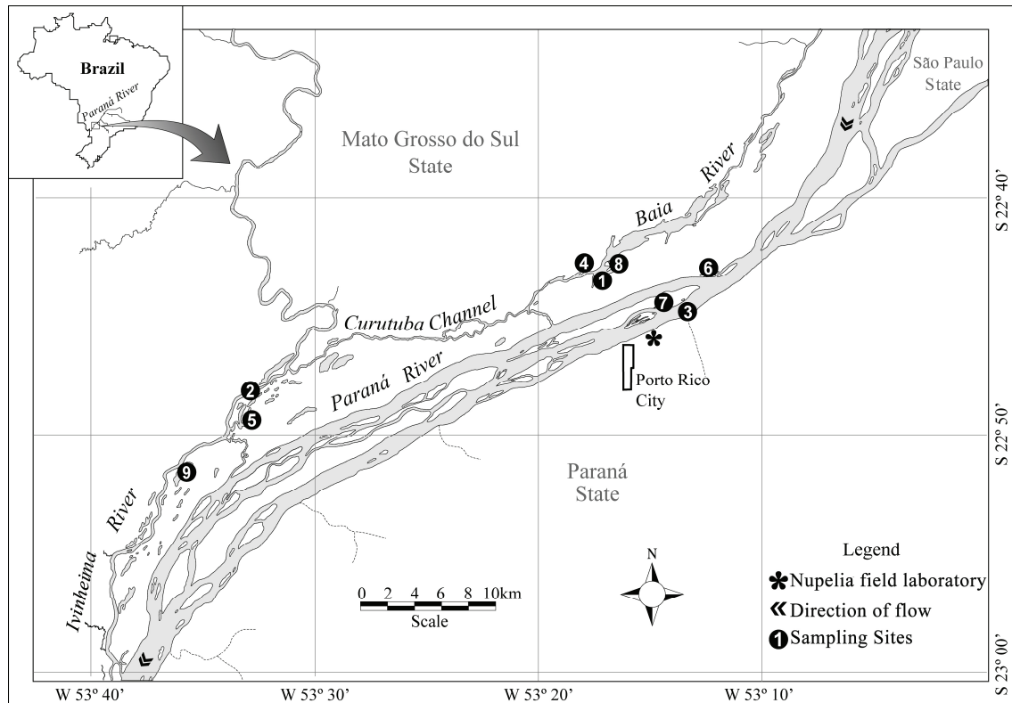
Figure 1. Study area and location of the sampling sites (Baia River – 1; Ivinheima River – 2; Paraná River – 3; Guaraná Lagoon – 4; Patos Lagoon – 5; Garças Lagoon – 6; Ressaco do Pau Veio Lagoon – 7; Fechada Lagoon – 8; Ventura Lagoon – 9) on the upper Paraná River floodplain.
