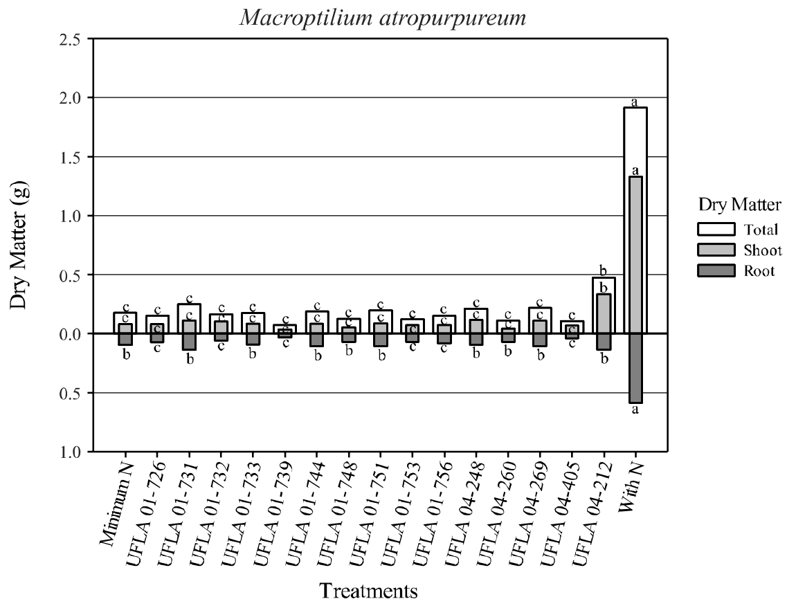
Figure 1 - Shoot dry matter, root dry matter and total dry matter (g), with coefficient of variation (CV) of 45.3, 23.3 and 31.4%, respectively, of Macroptilium atropurpureum , with the different treatments: treatments with individual inoculation with strains (Table 1 indicates the identification of strains); and two treatments without inoculation: one containing high mineral N concentration - 52.5 mg L -1 (With N), and another containing low mineral N concentration- 5.25 mg L -1 (Minimum N) concentration. All inoculated treatments received low mineral N concentration- 5.25 mg L -1 . Columns followed by the same letter do not statistically differ by the Scott-Knott test at 5% probability
