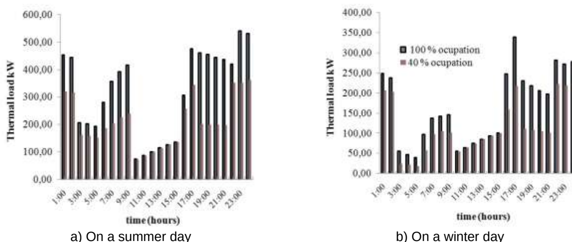
Fig. 6: Thermal loads Vs. Occupations' profiles. Source: Authors
