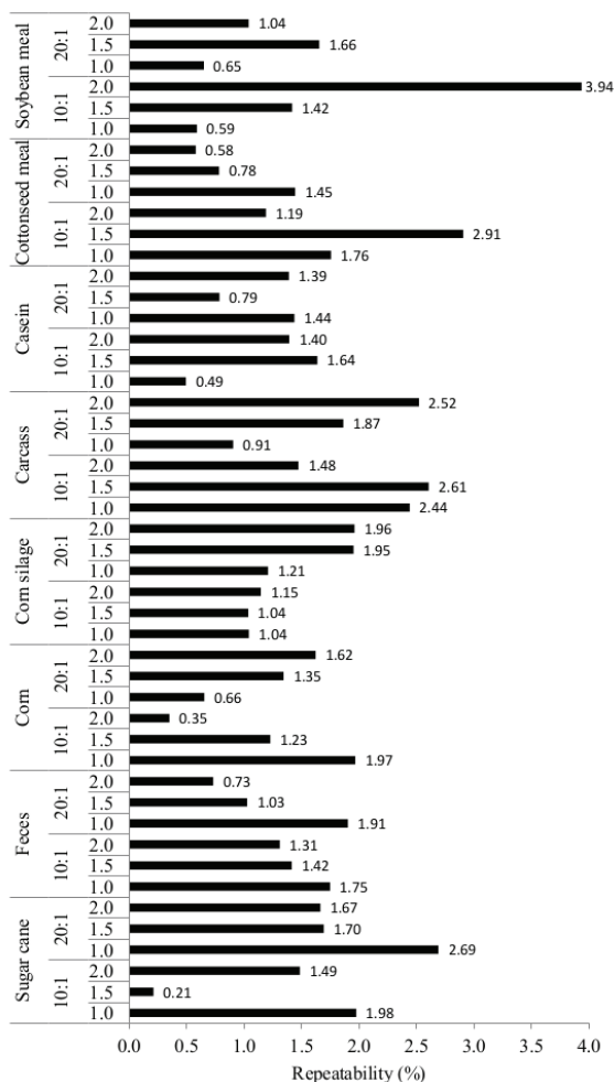
Figure 1. Standardized repeatability for the different low- and high-nitrogen materials according to the salt-to-metal catalyst ratios and amounts of digestion mixture.
