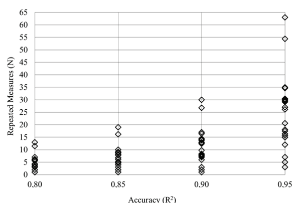
Figure 2. Estimated number of repeated measures for total dry matter yield (DMV) of P. maximum for four levels of accuracy with data from 6 different studies by Martuscello et al. (2007, 2015), Léo et al. (2008), Torres et al. (2016), Exp. 1, and Exp. 2.
