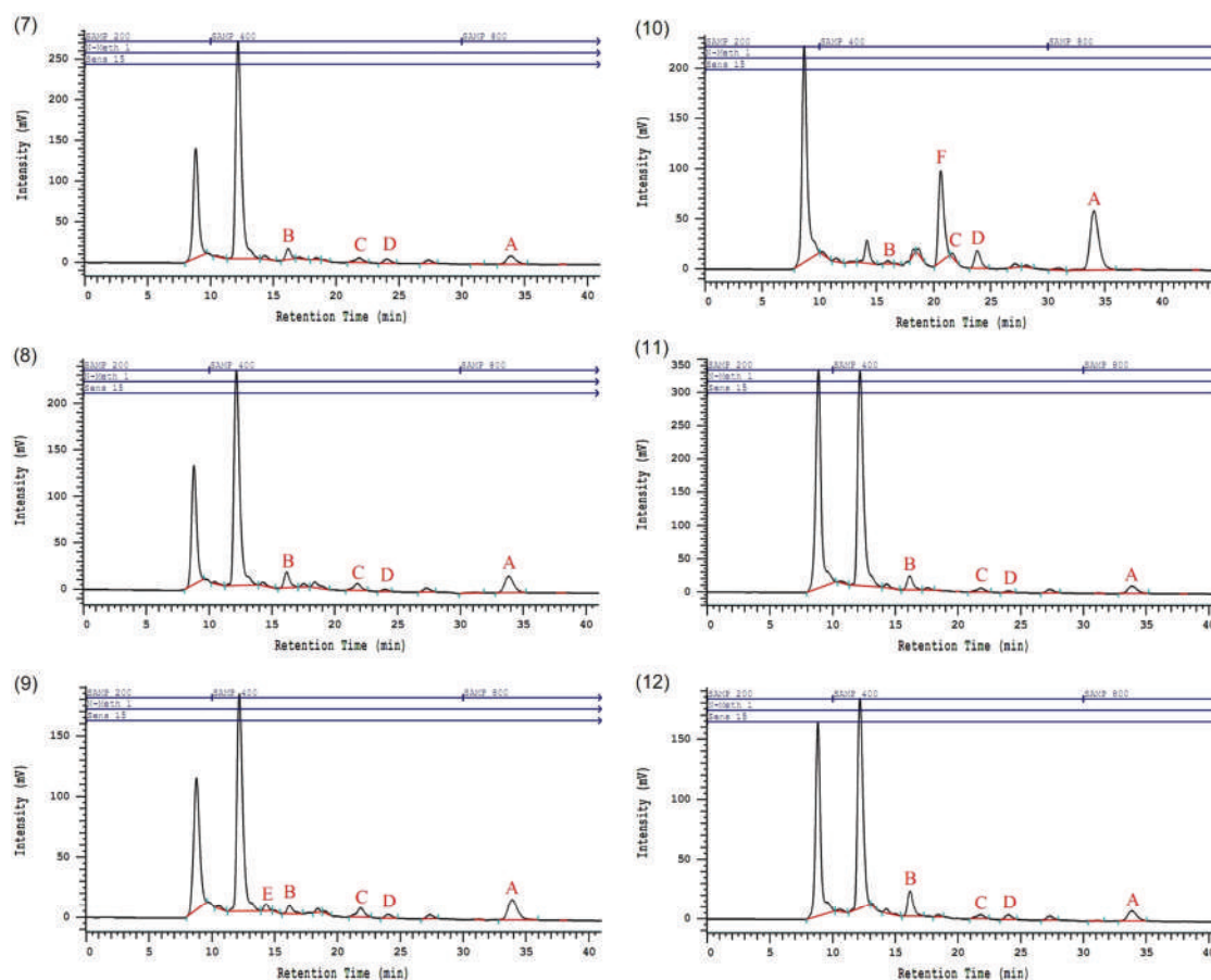
Figure 3. Chromatogram: (7) Cedrela fissilis Vell; (8) Ocotea porosa ; (9) Laurus nobilis ; (10) Balfourodendron riedelianum ; (11) Pinus elliotti ; (12) Brosimum spp. Identification of compounds: (A) Ethanol; (B) Fructose; (C) Glycerol; (D) Acetic acid; (E) Glucose; (F) Lactic acid. Transgenomic column (ICE-ION 300); flow rate 0.5 mL min -1 ; mobile phase 8.0 mM H 2 SO 4 .
