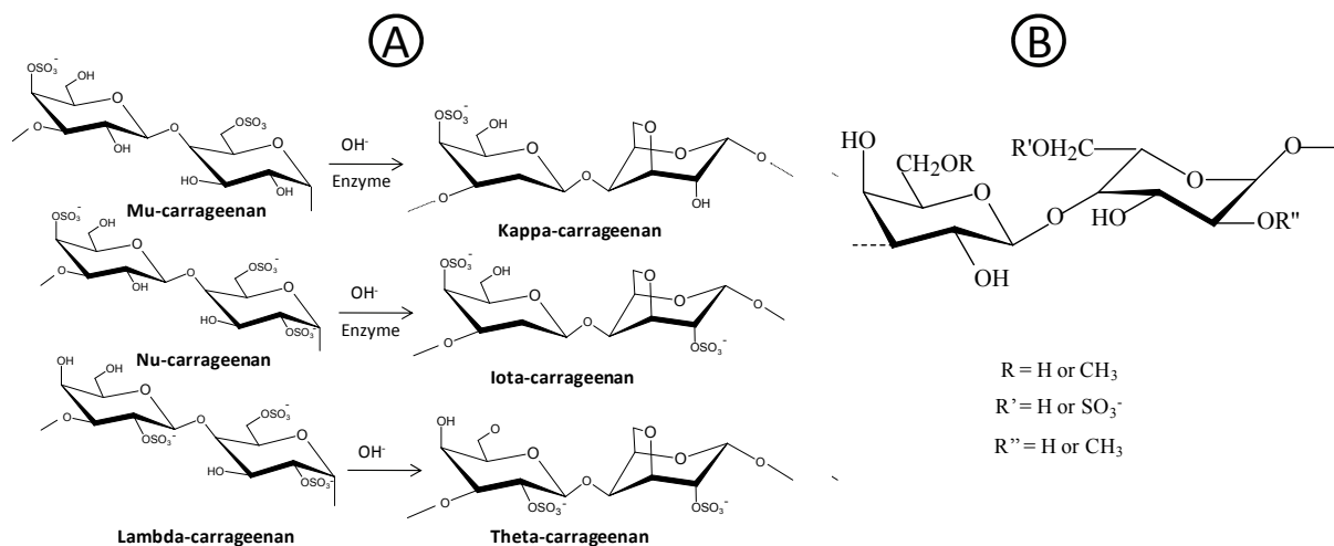
Figure 1. Chemical structures of Mu ( \mu )-, (Nu ( \nu )-, Lambda ( \lambda )-, Kappa ( \kappa )-, Iota ( i )- and Theta ( \theta )-carrageenans (A) and agar (B). Polysaccharides are formed by alternate units of D-galactose and 3,6-anhydro-D-galactose (A) or D-galactose and 3,6-anhydro-L-galactose (B) joined by \alpha -1,3 and \beta -1,4-glycosidic linkage.
