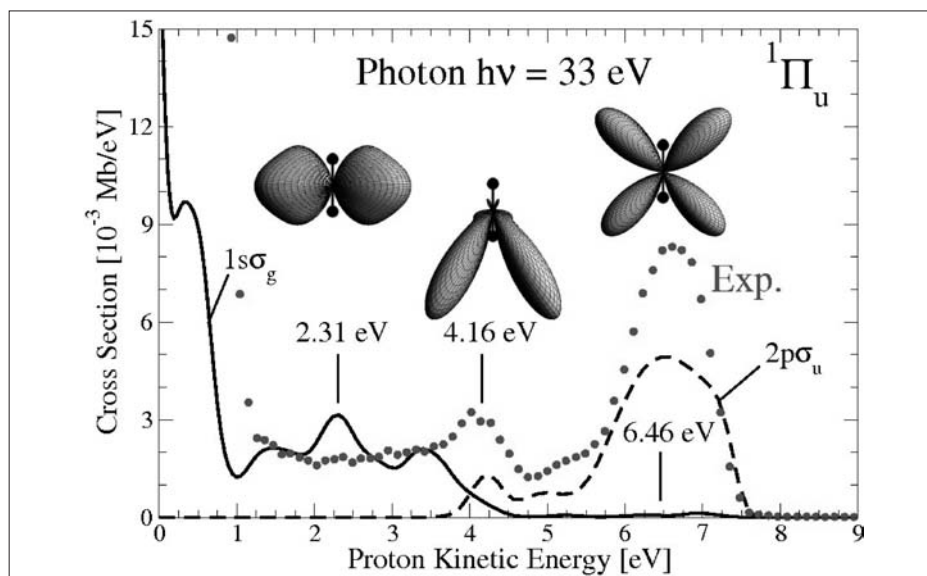
Figure 2. {}^1\Pi_u proton kinetic energy distribution (KED) in the dissociative ionization of H_2 for protons detected at 90^\circ with respect to the laser polarization axis and photon energy 33 eV. Solid line: contribution from the {}^2\Sigma_g^+(1s\sigma_g) ionization channel; dashed line: contribution from the {}^2\Sigma_u^+(2p\sigma_u) ionization channel; dots: experimental data from Ref. [1] must be compared with the sum of both contributions. Correct electron angular distributions (EADs) are in display for three selected proton energies. In the EADs the laser polarization vector is perpendicular to the molecular axis within the plane of the figures and the proton is pointing upwards. Mb stands for Megabarn (1 barn = 1024 \text{ cm}^2 ).
