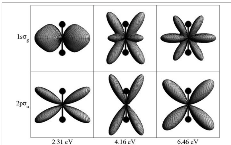
Figure 3. Electron angular distributions (EADs) contributed from the {}^2\Sigma_g^+(1s_g) + e(\pi_u) and the {}^2\Sigma_u^+(2p_s_u) + e(\pi_g) ionization channels for the three proton energies quoted in Figure 2. Explanations for EADs in Figure 2 also apply here.
