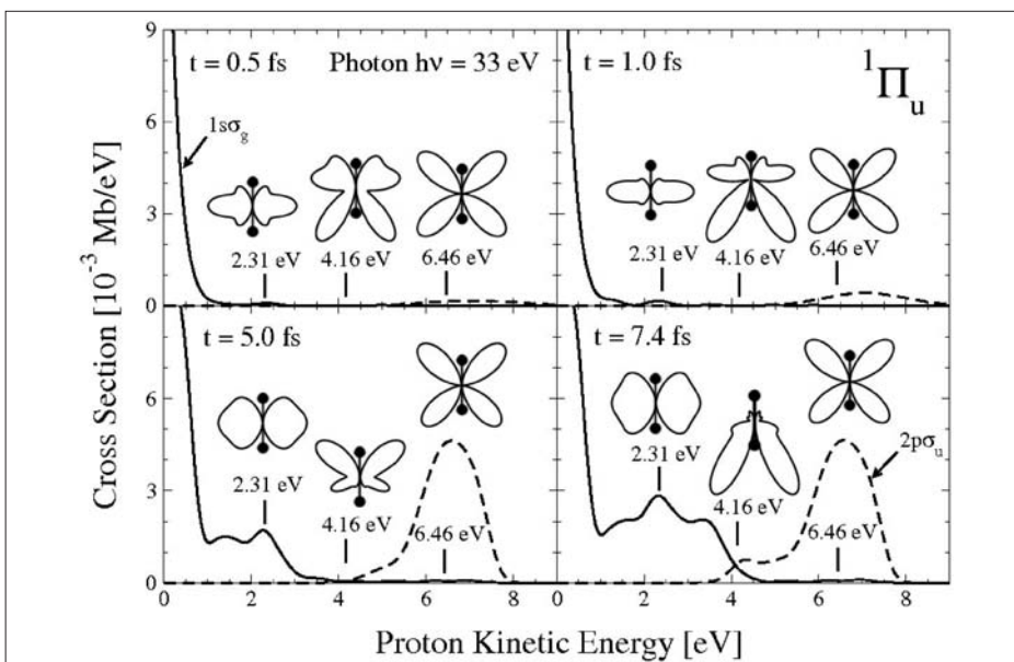
Figure 4. Time evolution for the {}^1\Pi_u proton kinetic energy distribution (KED) and for the electron angular distributions (EAD) at three proton energies in the dissociative ionization of H_2 mediated by a laser pulse with duration of T = 10 fs and photon energy \omega = 33 eV. The propagation time for each snapshot is indicated. Results for t = T = 10 fs are those included in Figure 3.
