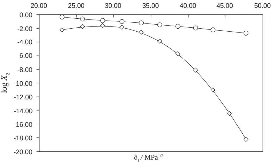
Figure 2. Experimental solubility (○) and calculated solubility according to the regular solutions model of Hildebrand (◇) of ACP as a function of the solubility parameter of the solvent mixtures at 298.15 K.
