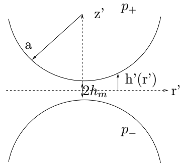
Fig. 1 – Slide view of the two identical particles under study.
