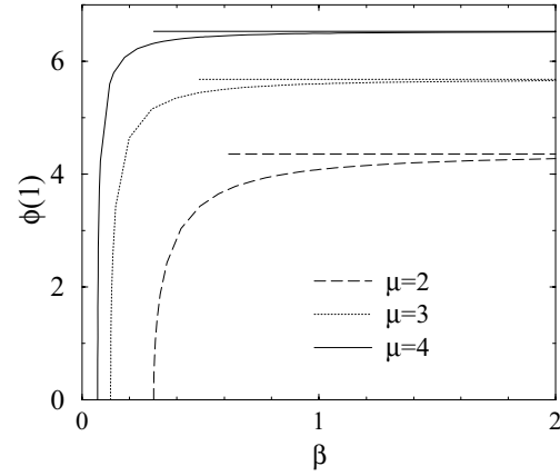
Fig. 2 – Surface potential of an anti-symmetric solution \phi(1) at \zeta = 1 versus dimensionless parameter \beta . The dotted lines indicate an asymptotic value which can be computed (Cf see Plouraboué and Chang (2009) for more details on this point).
