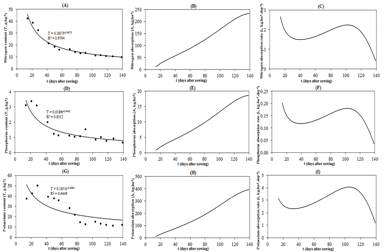
Figure 3 - Macronutrient content of the whole plant ( T , g.kg^{-1} ), total absorption ( A , kg.ha^{-1} ) and absorption rate ( \lambda , kg.ha^{-1}.day^{-1} ) for nitrogen ( a , b and c ), phosphorus ( d , e and f ) and potassium ( g , h and i ) in the maize (hybrid DKB 390 PRO 2) crop (weighted average of all organs) in relation to the number days after sowing ( t , days after sowing). Piracicaba (SP), Brazil.
