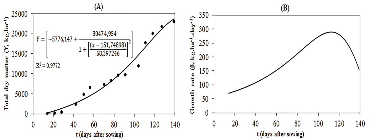
Figure 2 - Total dry matter (Y, kg.ha -1 ) (a) and growth rate (β, kg.ha -1 .day -1 ) (b), of the maize crop (hybrid DKB 390 PRO 2), as a function of time (t, days after sowing - DAS). Piracicaba (SP), Brazil.
