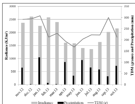
Figure 1 - Irradiance levels and precipitation in relation to increases in total dry matter (TDM) of Martianthus leucocephalus (Mart. Ex Benth.) JFB Pastore, exposed to the edaphoclimatic conditions of Feira de Santana, Bahia State, Brazil.
