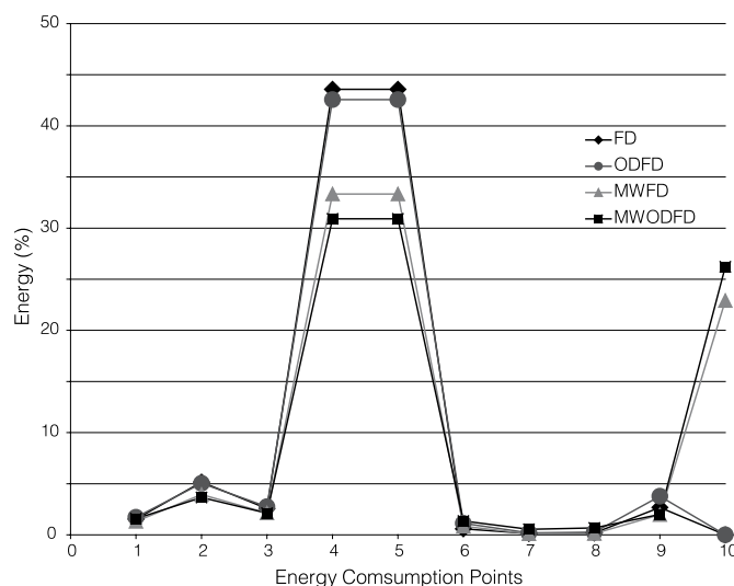
Figure 3. Energy consumption (%) during the different drying treatments.
