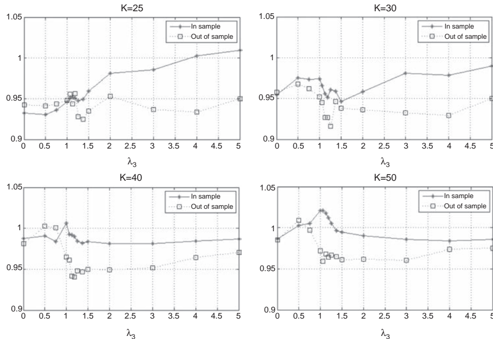
Fig. 19. In-sample and out-of-sample beta (as a function of \lambda_3 ) for different values of K and y = (y^{mkt}, y^\alpha, y^\beta) .
