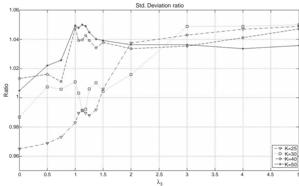
Fig. 10. Ratio of standard deviations of the tracking portfolio with respect to the index for different values of K and \lambda_3 using (y^{mkt}, y^\alpha, y^\beta) as characteristics.
