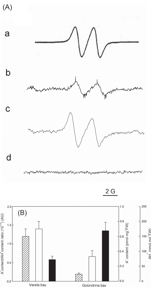
Fig. 5: A: EPR detection of ascorbyl radical in liver of O. nigricans from different sampling sites: (a) computer-simulated EPR spectra employing the following spectral parameters g = 2.005 and a_H = 1.8 G, (b) typical EPR spectra from Golondrina bay, (c) typical EPR spectra from Varella bay and (d) EPR spectra of dimethyl sulfoxide (DMSO). B: A (□) and AH (■) contents and A/AH ratio (▨) in liver of O. nigricans from different sampling sites.
