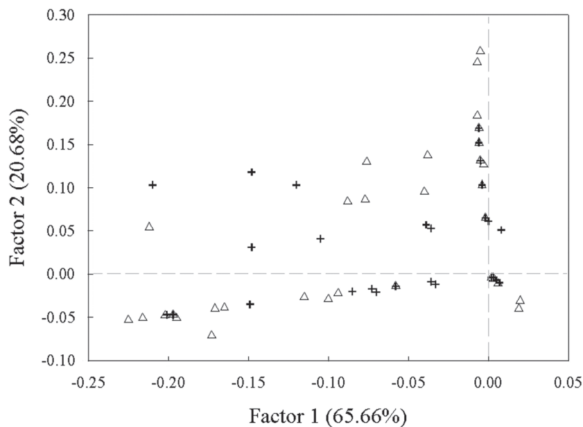
Fig. 3: Plot representing the first two factors of a principal components analysis performed on the diet composition of T. chiltoni (Δ) and T. areolatus (+), between 1994 and 2000 in all seasons. Percentage of the total variance of each factor is shown in parenthesis.
