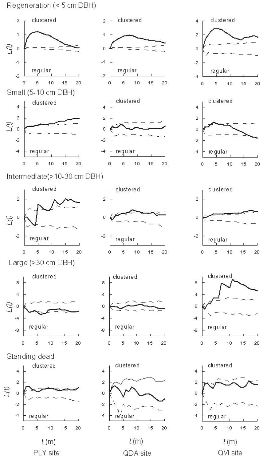
Fig. 3: Spatial distribution (function L(t) ) of Myrceugenia fernandeziana trees of different diameter categories. The dashed lines represent the confidence envelopes for a random distribution ( \alpha = 99\% ). See Fig. 1 for information about the sites.
