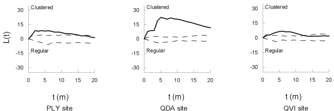
Fig. 4: Spatial pattern (function L(t) ) for all individuals of Fagara mayu and Drimys confertifolia . The dashed lines represent the confidence envelopes for a random distribution ( \alpha = 0.99 ). See Fig. 1 for information about the sites.
