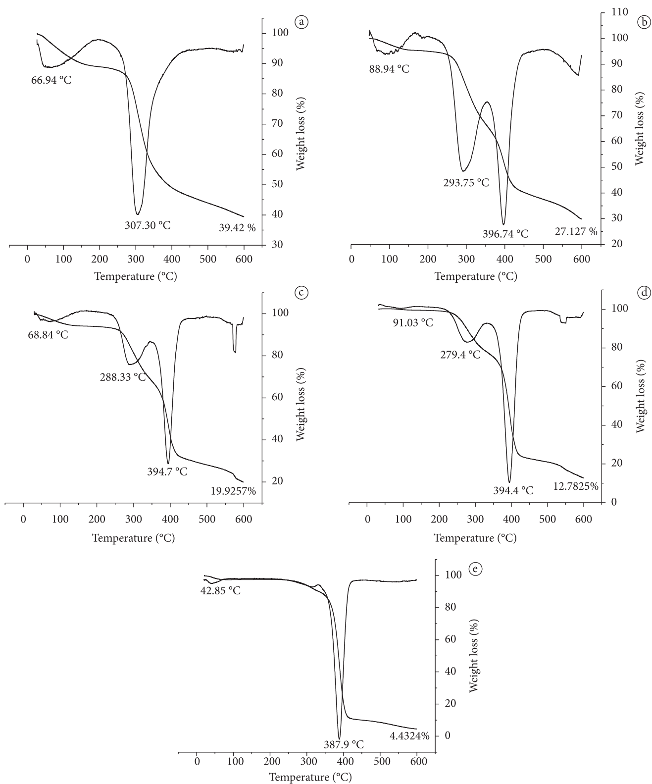
Figure 3. Thermogravimetric analysis of chitosan/HPMC films (A:Q100/HPMC0; B:Q70/HPMC30; C:Q50/HPMC50; D:Q30/HPMC70, and E:Q0/HPMC100).
