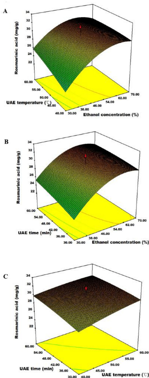
Figure 2. Response surface plots for the effect of (A) temperature and ethanol concentration (B) time and ethanol concentration and (C) time and temperature on the rosmarinic acid content (RA).
