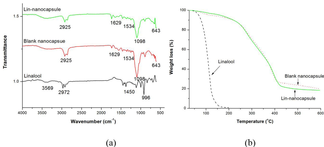
Figure 3. FTIR spectra (a) and Thermogravimetric analysis diagram (b) of linalool, Lin-nanocapsules and blank nanocapsules.
