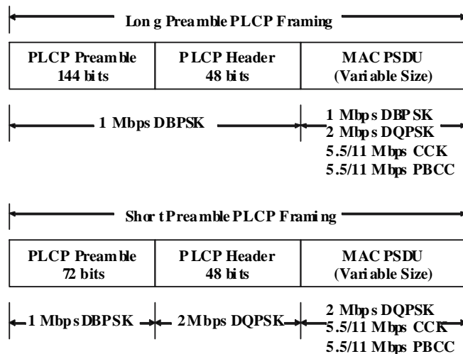
Figure 2. ERP-DSSS/CCK PHY layer PPDU framing
