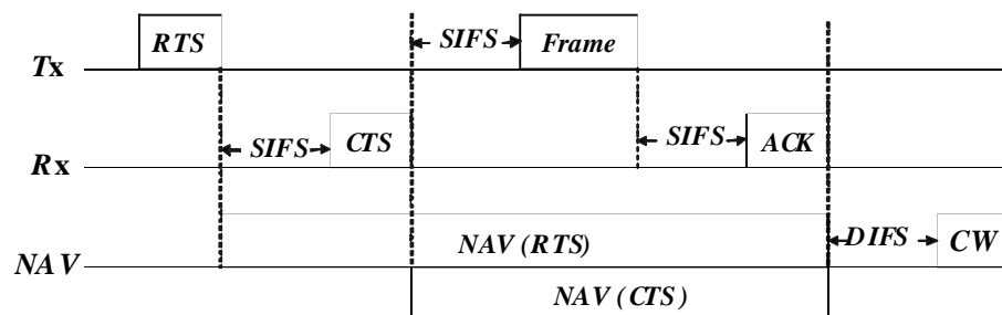
Figure 4. RTS/CTS protection mechanism
