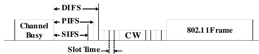
Figure 1. Illustration of the inter-frame spacing in 802.11
