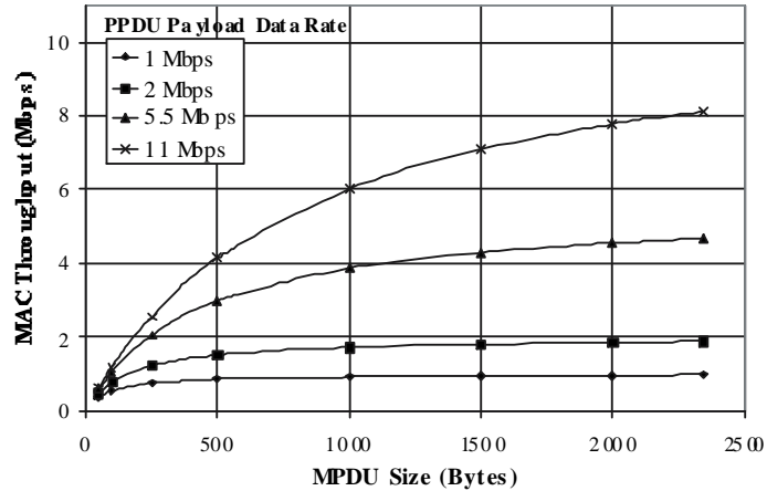
Figure 6. ERP-DSSS/CCK MAC Throughput (Long Preamble)
