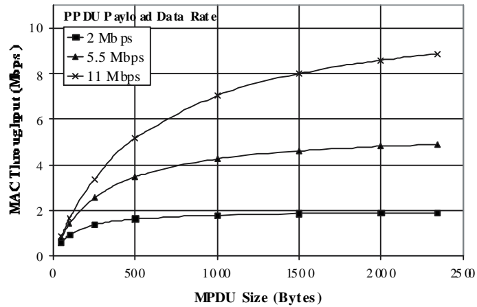
Figure 7. ERP-DSSS/CCK MAC Throughput (Short Preamble)
