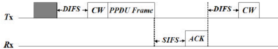
Figure 5. PPDU transmission time diagram
