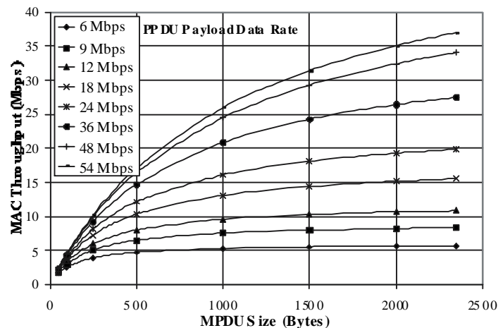
Figure 12. ERP-OFDM MAC Throughput (Time slot = 9 \mu s )
