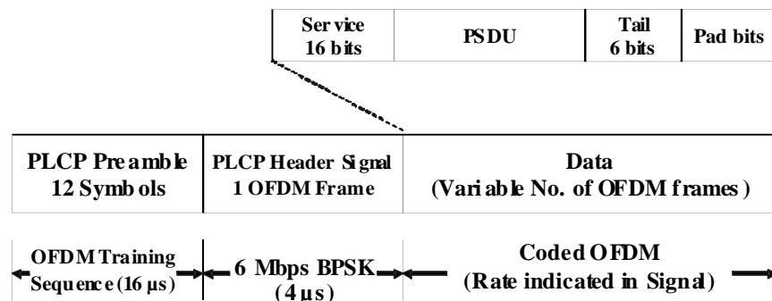
Figure 3. ERP-OFDM PHY layer PPDU framing
