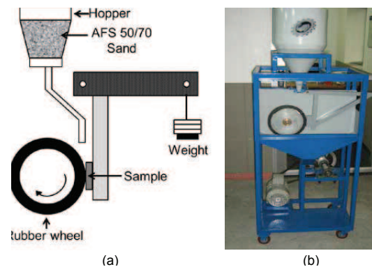
FIG. 2. (a) Schematic illustration for an abrasion system according to ASTM G-65 and (b) the abrasive wear test machine used in this study
