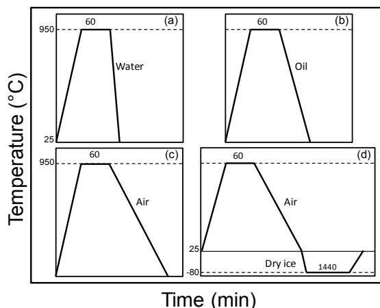
FIG. 1. Heat treatment cycles with different quenching media: a) water, b) oil, c) air and d) air and dry ice
