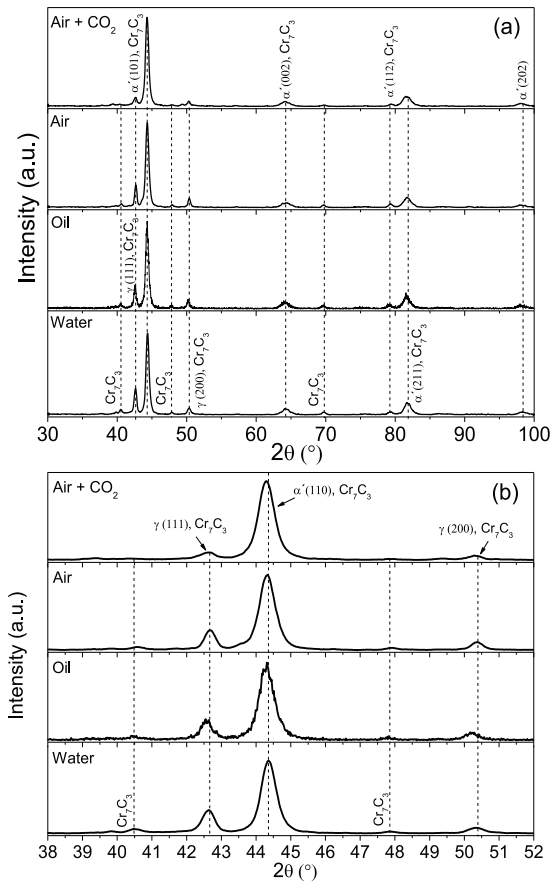
FIG. 6. XRD of the high chromium iron cast subjected to different heat treatments
