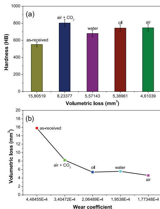
FIG. 7. Correlation between hardness and a) volumetric loss and b) wear coefficient
