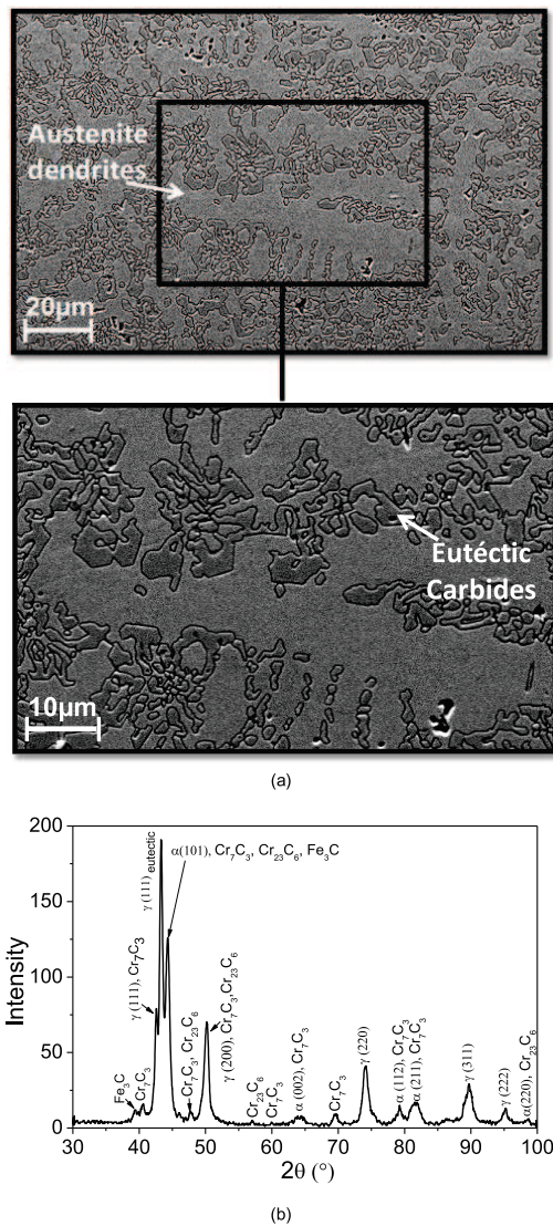
FIG. 4. (a) Scanning electron microscopy and (b) XRD of the as-received high chromium cast iron
