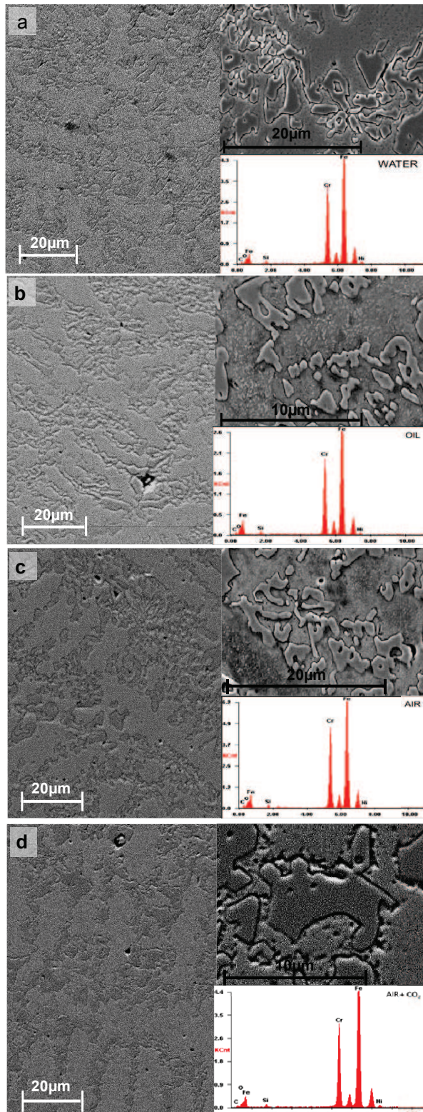
FIG. 5. SEM microstructures of samples quenched in a) water, b) oil, c) air and d) air and dry ice
