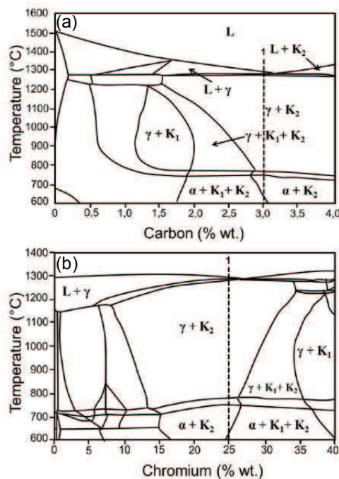
FIG. 3. Equilibrium phases calculated by ThermoCalc software [2]: (a) Fe-C system with 25% Cr and (b) Fe-Cr system with 3% C.
