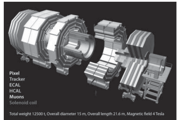
Figure 3. The CMS detector (layout).
