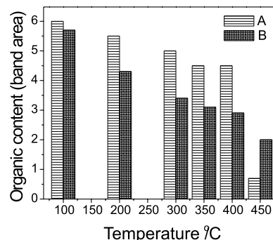
Figure 6: Relative remaining organic content of the xerogel samples A and B calculated from the band areas of the infrared ring mode at 1517 \text{ cm}^{-1} , after thermal treatment at each temperature.
