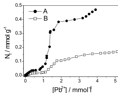
Figure 5: Metal ion adsorption isotherms of xerogel samples A and B, obtained at 25 °C, in aqueous solution for \text{Pb}^{2+} .
