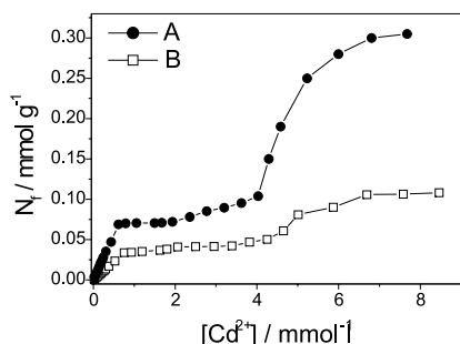
Figure 4: Metal ion adsorption isotherms of xerogel samples A and B, obtained at 25 °C, in aqueous solution for \text{Cd}^{2+} .
