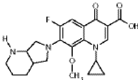
Figure 1. Structure of moxifloxacin.
