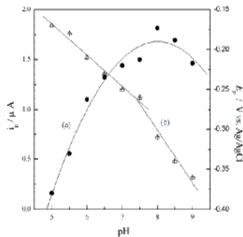
Figure 3. Influence of pH on the peak current (a) and peak potential (b) response for 5.00 \times 10^{-6} mol l^{-1} MOXI in the presence of 5.00 \times 10^{-6} mol l^{-1} Cu(II) in Phosphate buffers (pH 5.0–9.0). Other parameters: Fig. 2.
