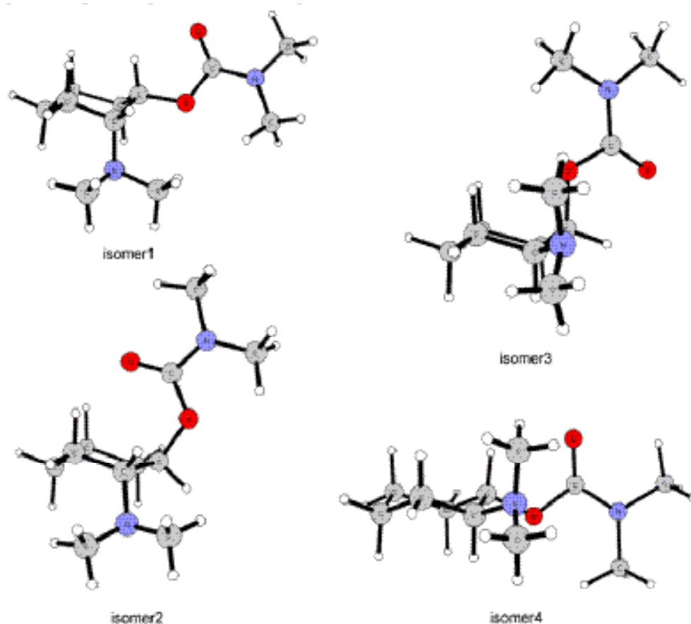
Figure 1. Optimized geometries of molecular models of four different isomers of 2- N,N -dimethylaminecyclohexyl 1- N',N' -dimethylcarbamate.
