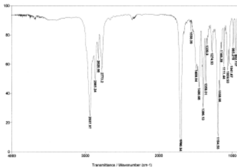
Figure 2. Experimental IR spectrum of isomer 3 in 3.00 X 10 -2 M CCl 4 solution.
