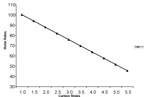
Figure 4b. Production of PCDD/F's upon the variation of carbon availability with chlorine and hydrogen
