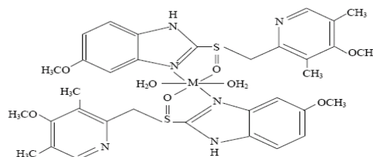
Figure 4: Structure of OME Complex with Mn(II),Fe(II),Cu(II),Co(II),Ni(II) Metals
